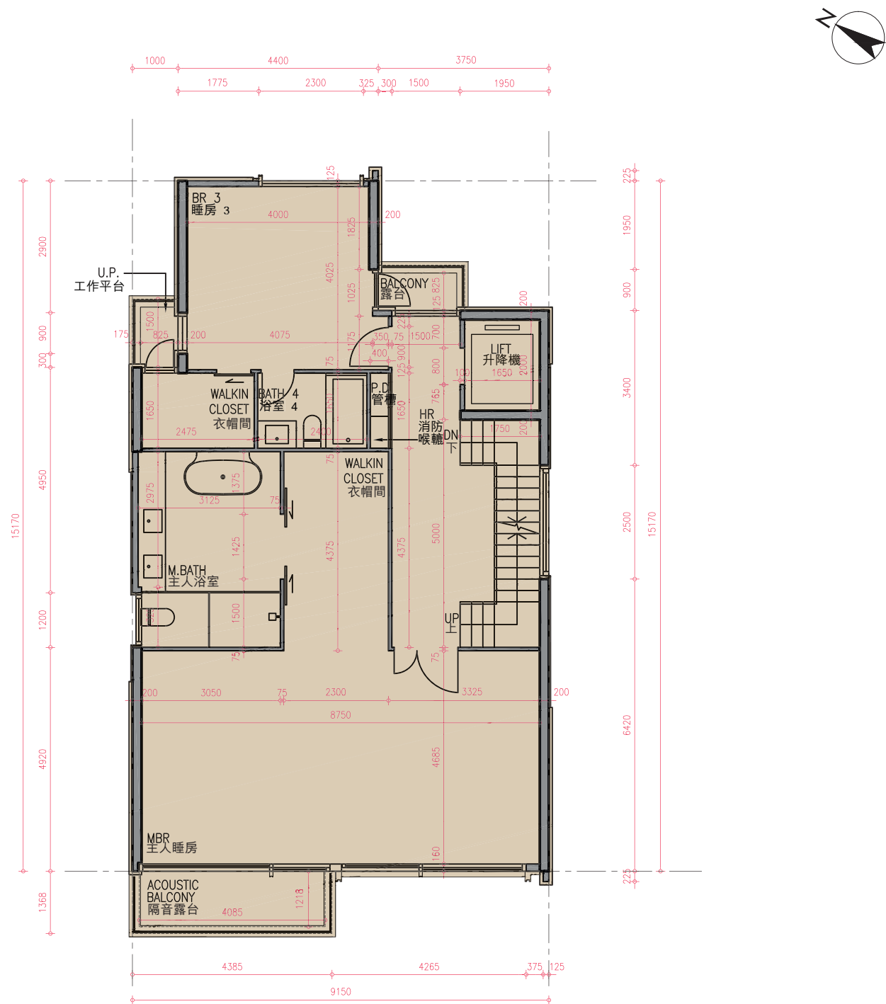
1 號洋房2樓平面圖 HOUSE 1 SECOND FLOOR PLAN
